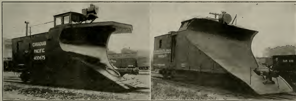
SINGLE TRACK STEEL PLOW—CANADIAN PACIFIC RAILWAY. FULLER TYPE, SINGLE TRACK PLOW—PENNSYLVANIA LINES
